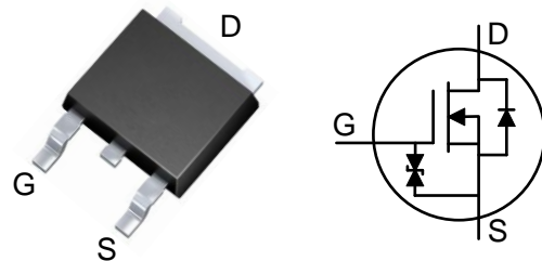
TO-252
