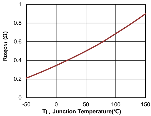
Figure 9. Drain-to-Source On-Resistance vs. Junction Temperature
